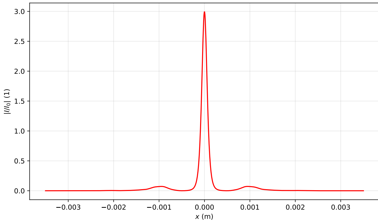
Intensity profile I(x, y = 0, z = 2.149)/I_0 , P_{in}=9.0P_{cr} , artificial time
